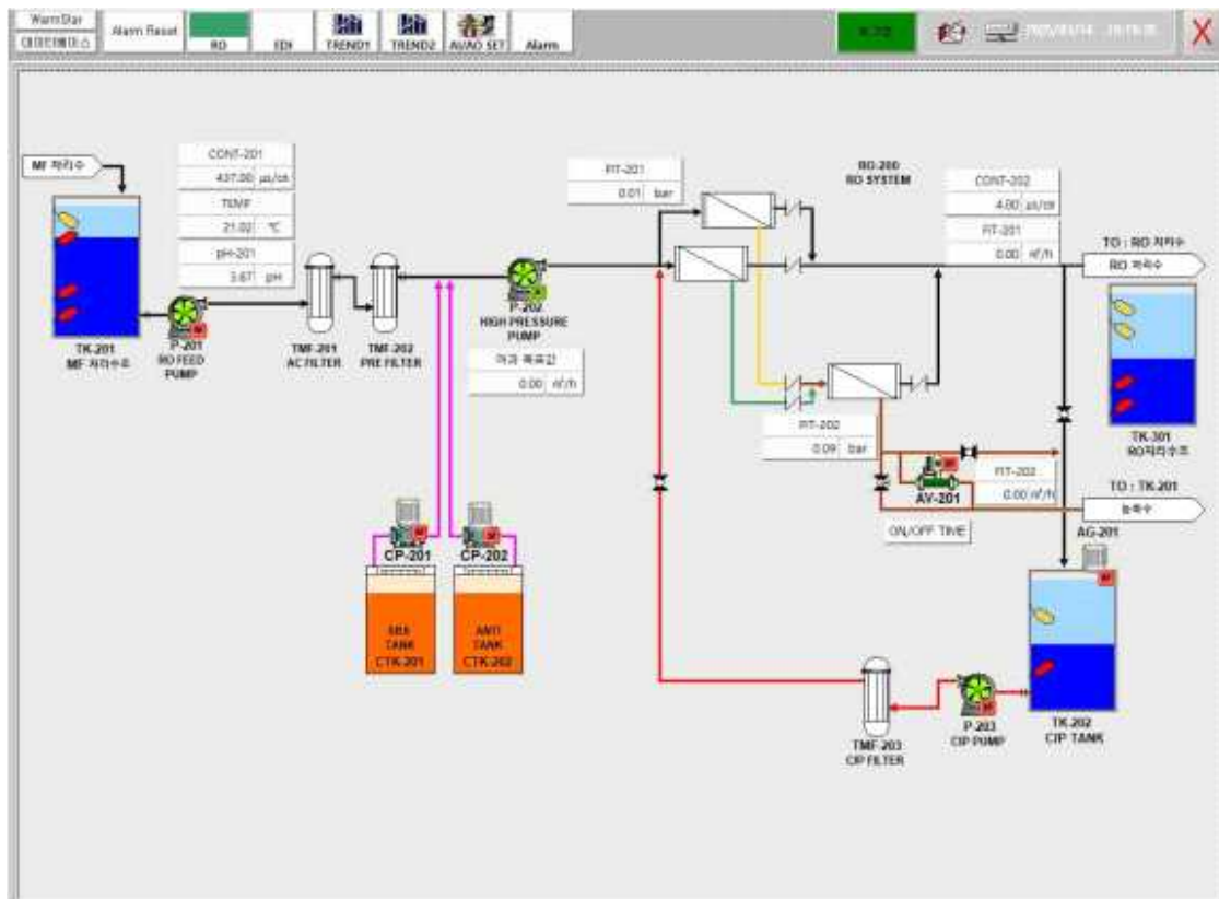
Figure 4. Back-end control panel initial screen (RO process)
