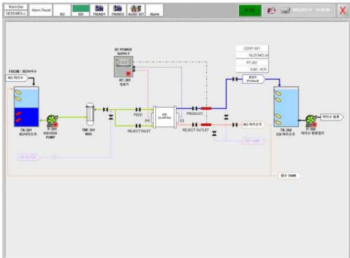
Figure 5. Back-end control panel initial screen (EDI process)
